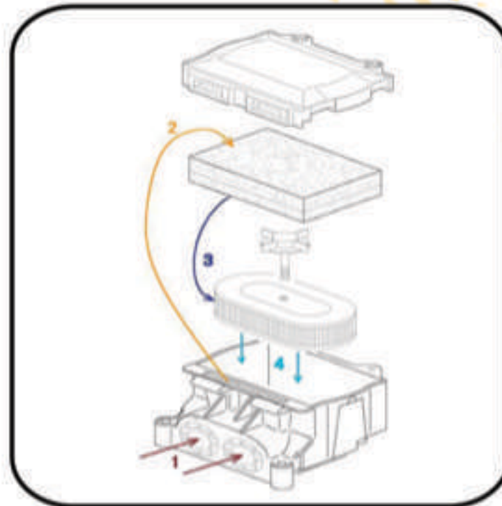
Air cleaner
