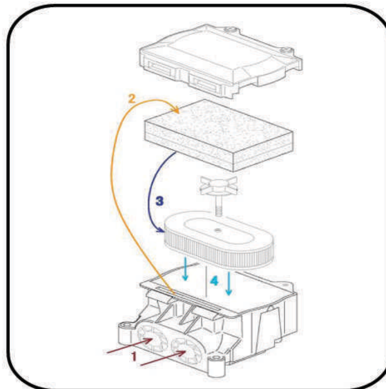
Air Cleaner
